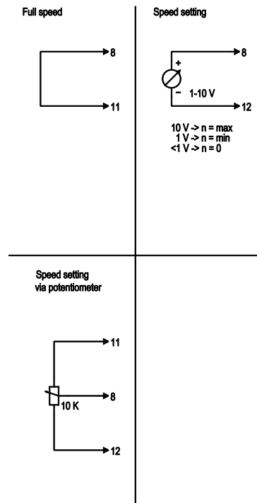
Customer circuit
